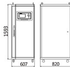
Power Amplifier SDA-3
