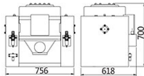
Shaker ET-2-230
