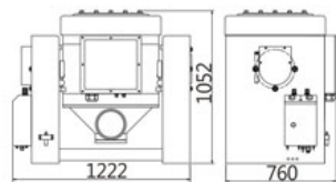
Shaker ET-20-445
