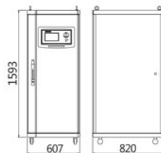
Power Amplifier SDA-2
