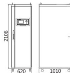
Power Amplifier SDA-50
