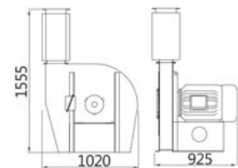
Blower B-7000
