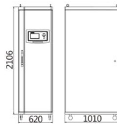
Power Amplifier SDA-60
